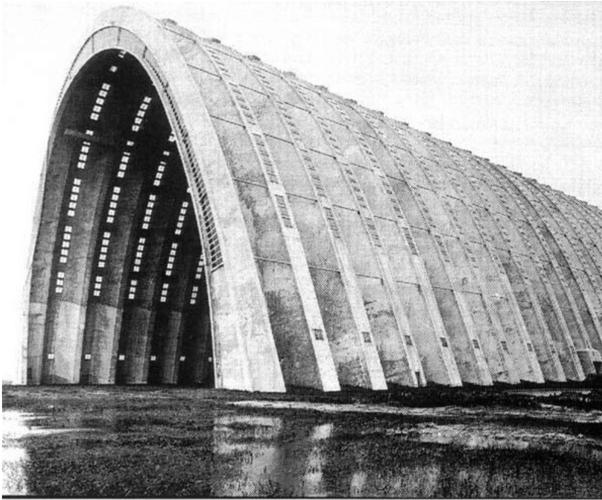
Orly Hanger -- Eugene Freyssinet (~1922)
